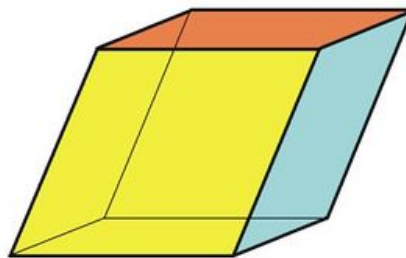
Rhombohedron
