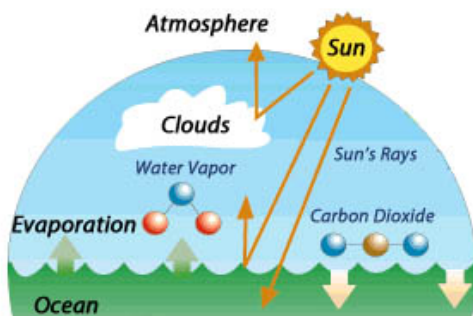
Gas Exchange Between Oceans and Atmosphere
