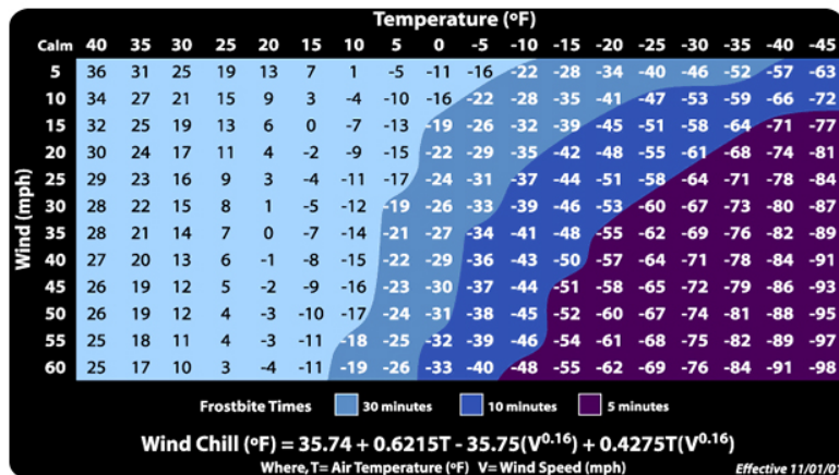
NWS Windchill Chart
