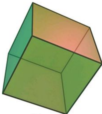
Cube
