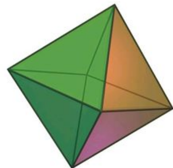
Octahedron
